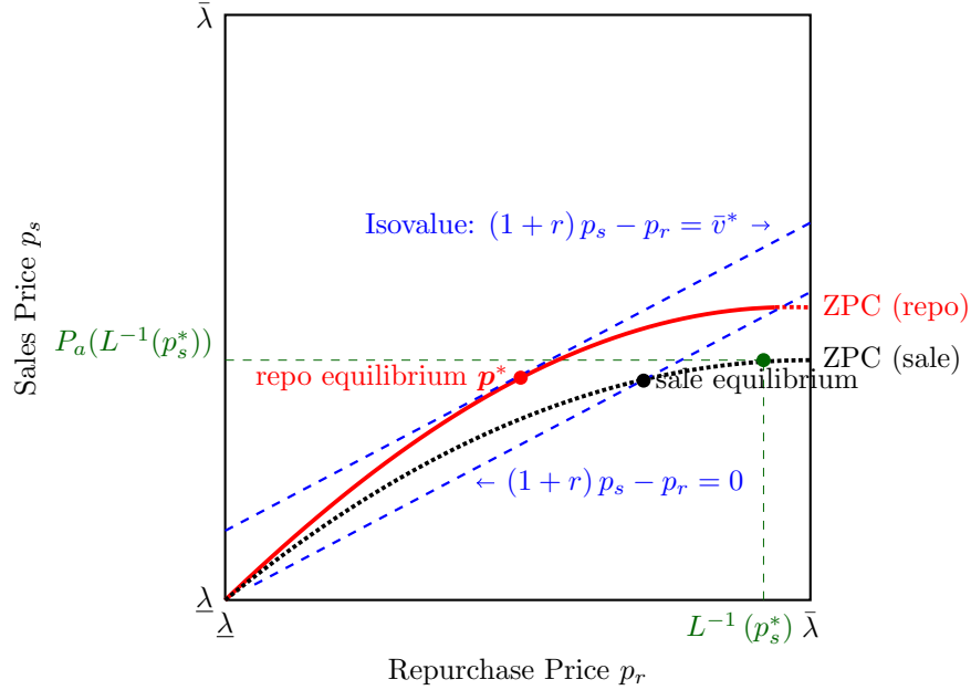
Figure 4: Comparison of repo contract vs. asset sales
